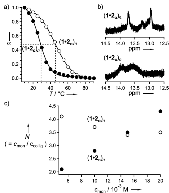
Figure 4. a) Plots of mole fraction of aggregates ( \alpha ) versus temperature for variable temperature UV/Vis spectra of (\mathbf{1} \cdot \mathbf{2}_{\text{o}})_n ( \circ ) and (\mathbf{1} \cdot \mathbf{2}_{\text{c}})_n ( \bullet ) in methylcyclohexane ( c = 1 \times 10^{-5} \text{ M} ). b) Comparison of ^1\text{H} NMR spectra of (\mathbf{1} \cdot \mathbf{2}_{\text{o}})_n in [\text{D}_{12}]\text{cyclohexane} ( c = 5 \times 10^{-4} \text{ M} ) before (upper panel) and after UV irradiation (lower panel). c) Plots of the aggregation number N (= c_{\text{mon}} / c_{\text{collig}}) determined by VPO versus stoichiometric concentrations ( c_{\text{mon}} ) of the components for (\mathbf{1} \cdot \mathbf{2}_{\text{o}})_n ( \circ ) and (\mathbf{1} \cdot \mathbf{2}_{\text{c}})_n ( \bullet ).
